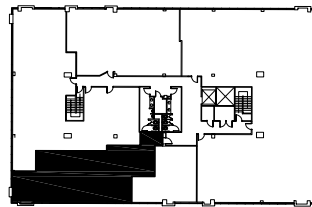
2ND FLOOR BUILDING "A"
